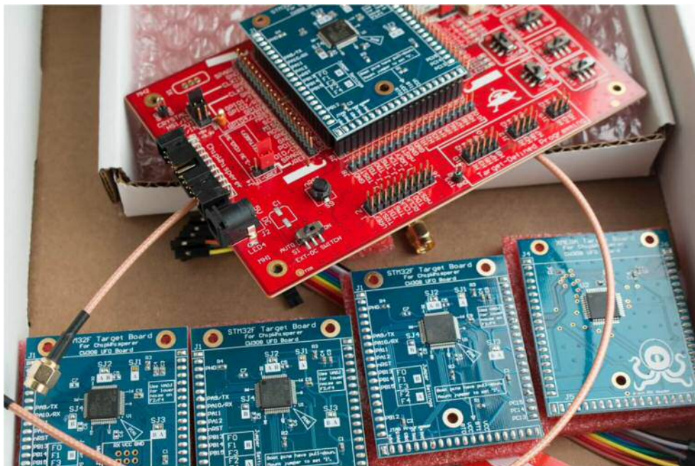
Abb. 2.1.1: ChipWhisperer
